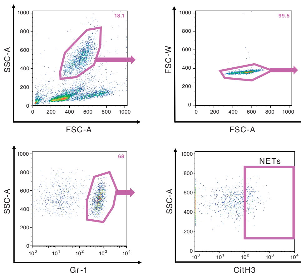
Fig. 1. Flow cytometry.
